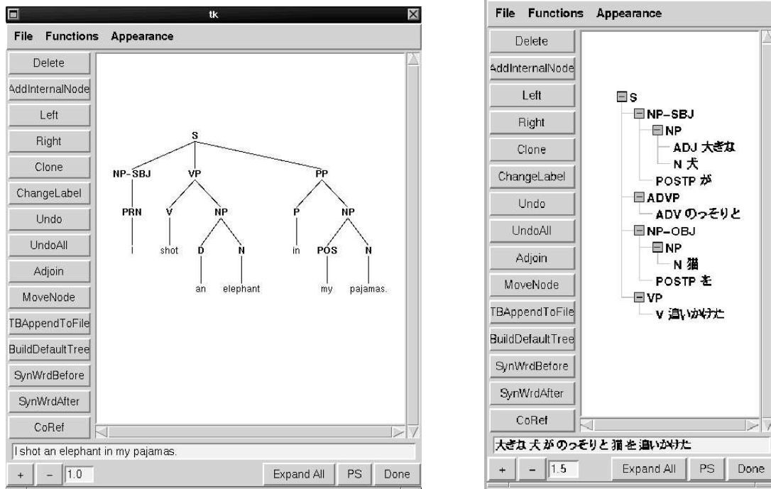
Figure 6: TreeTrans: Syntactic Transcription (Horizontal and Vertical Views)
