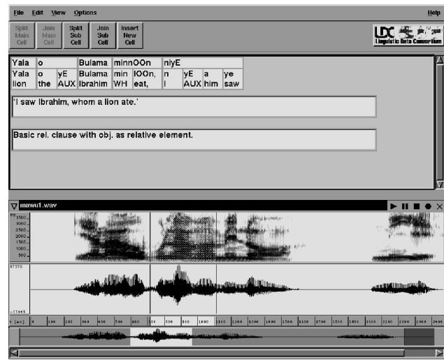
Figure 5: InterTrans, Interlinear Text Transcription
